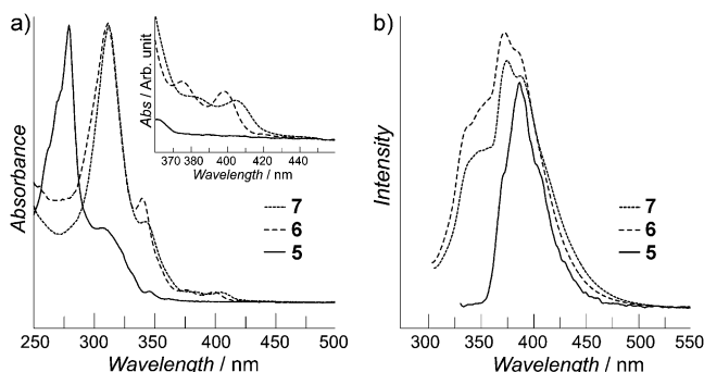
Figure 3. UV/Vis absorption (a) and emission spectra (b) of 6 and 7 measured in dichloromethane ( c = 10^{-5} \text{ mol L}^{-1} ) at 20 °C, along with those of 5 for comparison. The insert in (a) shows an expansion of absorption spectra in the long-wavelength region.
